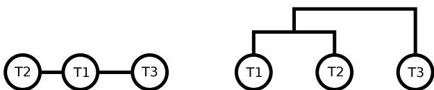
Figure 18 MSTs and time-series data. An example with a time-series data set of three samples (T1, T2, and T3) where the dissimilarity between T1 and T2 is the smallest, but between T2 and T3 is the largest. This phenomenon is depicted well by the MST (left), but not by the dendrogram (right) since T1 and T2 are part of the same sub-tree and could be re-ordered depending on the hierarchical clustering implementation.
